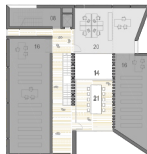
quarto piano cc.1.208
