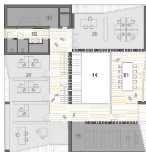
secondo piano second floor cc.1.290
